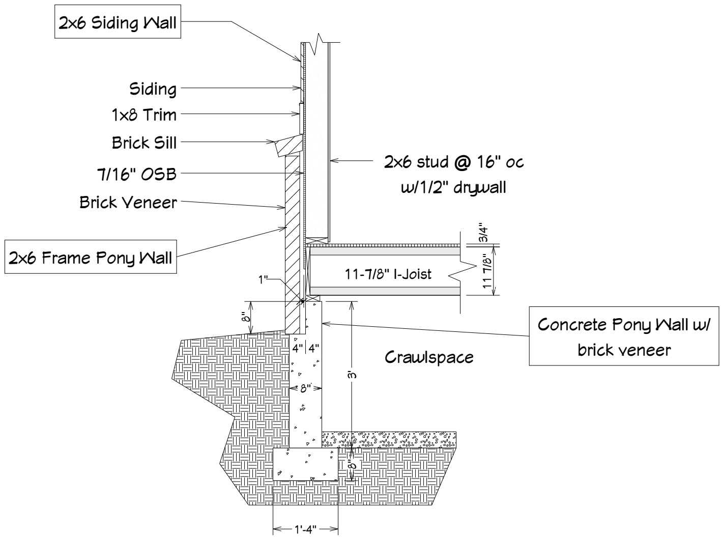
Foundation Section
