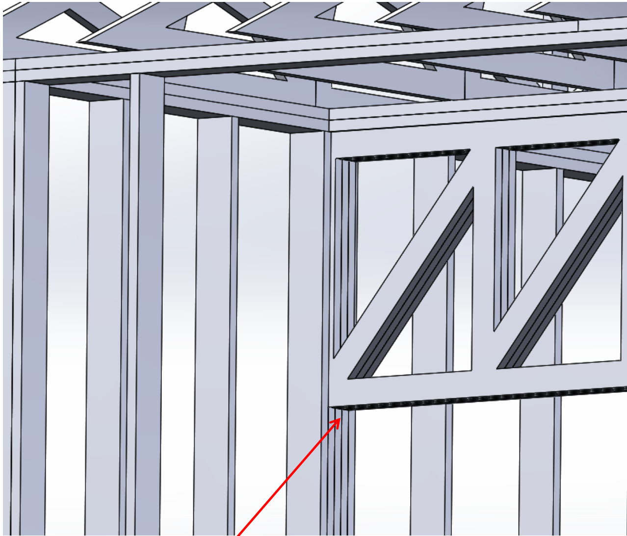
girder truss sitting on jack studs
