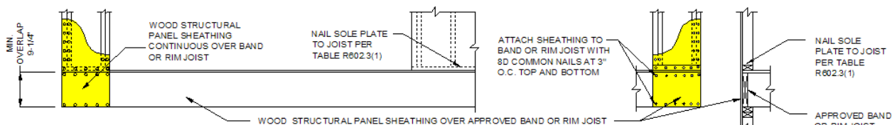
FRONT ELEVATION
