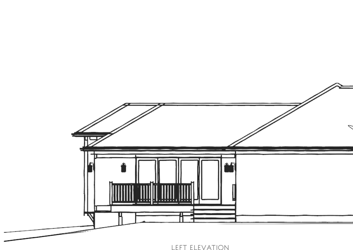
LEFT ELEVATION
